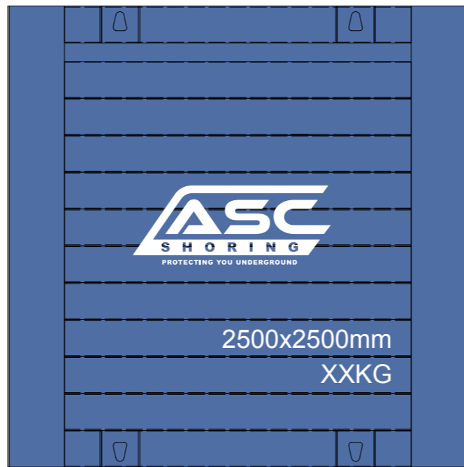
Front view (2500*2500*100)mm
