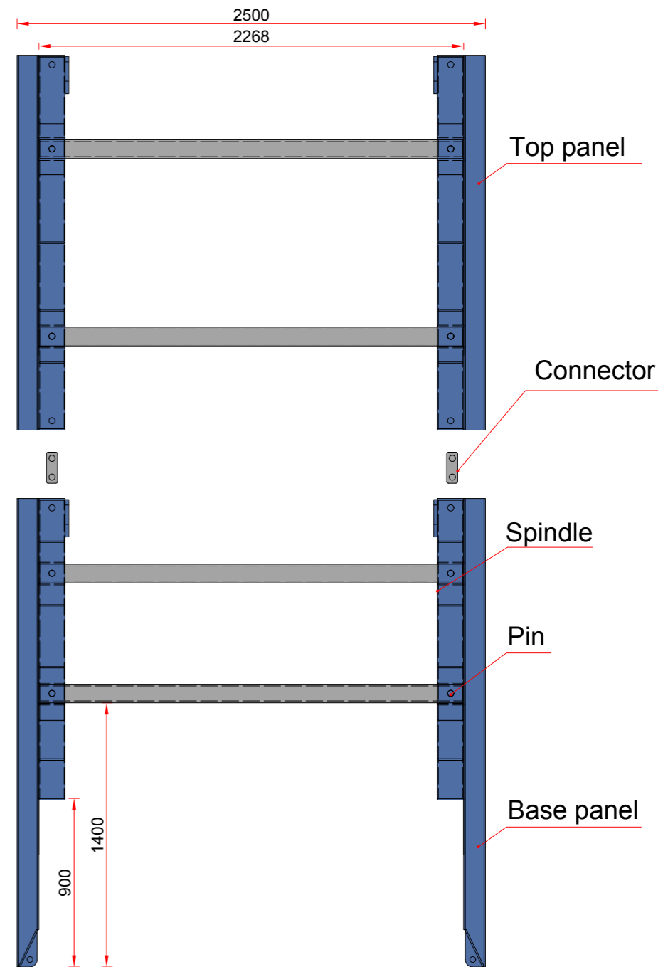
Built-up section
