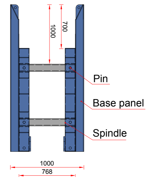
Built-up section
