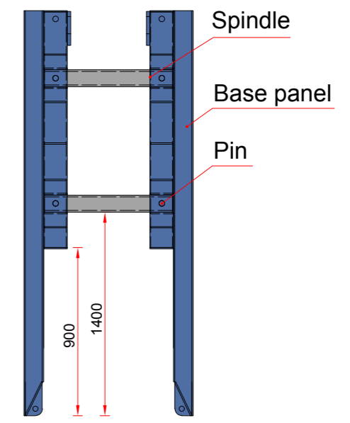
Built-up section
