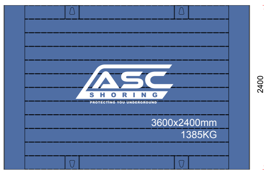
Front view (3600*2400*100)mm
