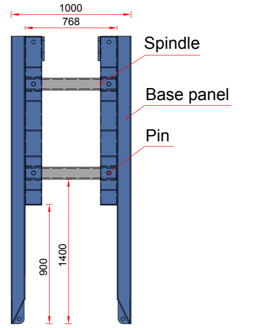
Built-up section
